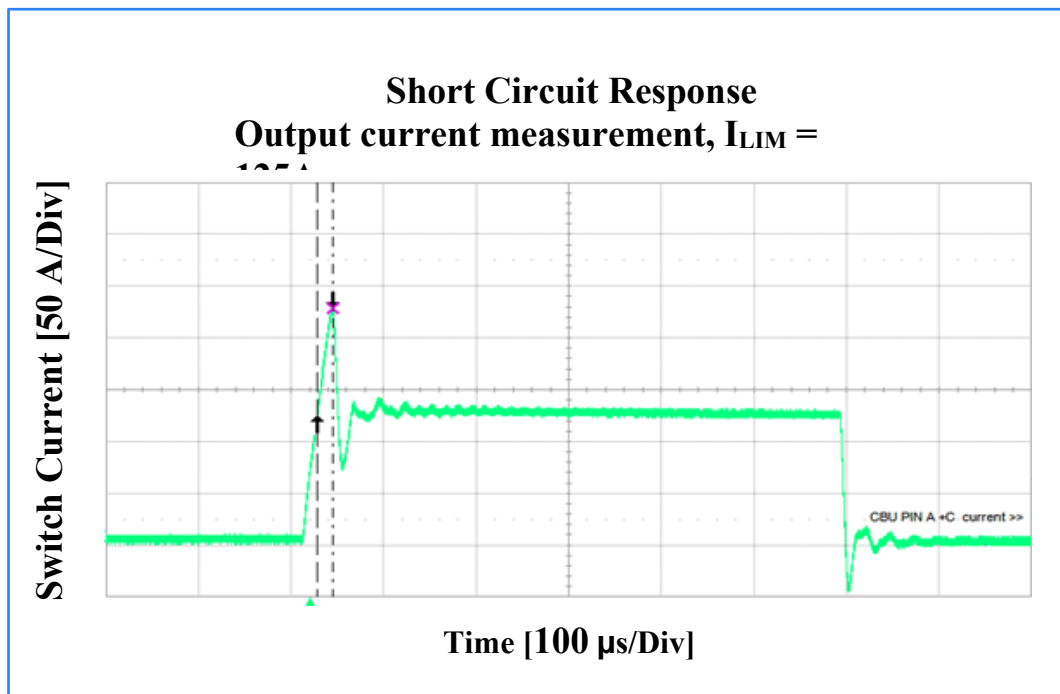
Figure 2 - Short Circuit Response
