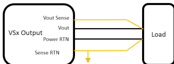
Figure 3: M4706 Sense line connection
