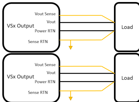
Figure 4: M4154 Sense line connection
